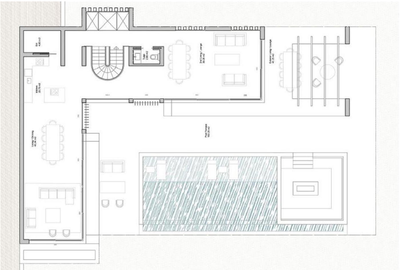
Ground floor
